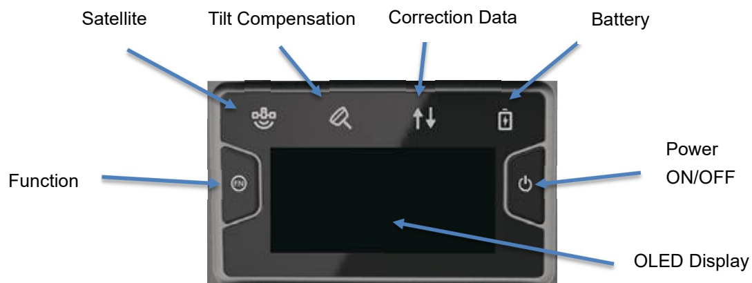
Figure 1.4 Buttons and Display on Oscar Ultimate
