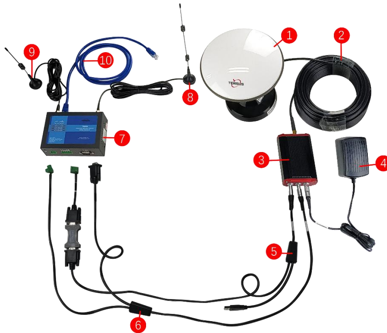
Figure 1 GeoBee System Set up
